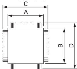
Outline IC Body Dimensions
